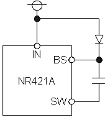
Fig. 8-3 Bootstrap Diode Connection 1
