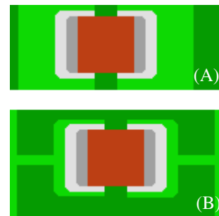
(A)···Recommended Pattern (B)···No good pattern example
