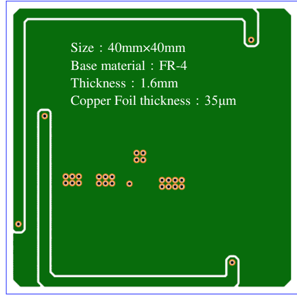
Fig. 8-8 Back side (see from surface)
