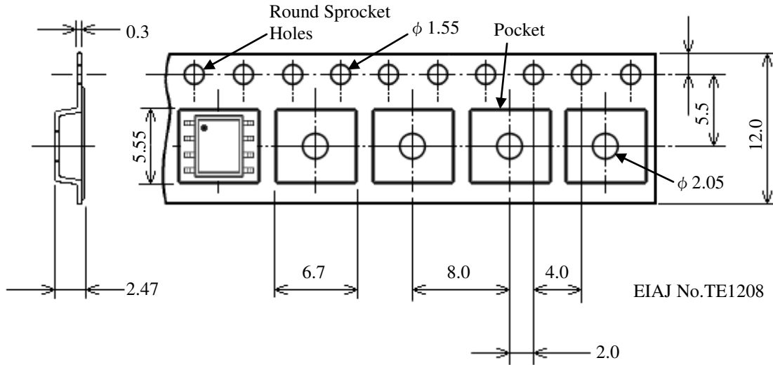
Fig. 10-1 Taping Outline
