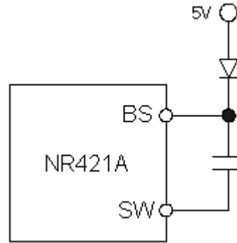
Fig. 8-4 Bootstrap Diode Connection 2
