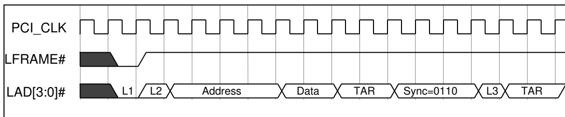
FIGURE 78 – I/O WRITE
