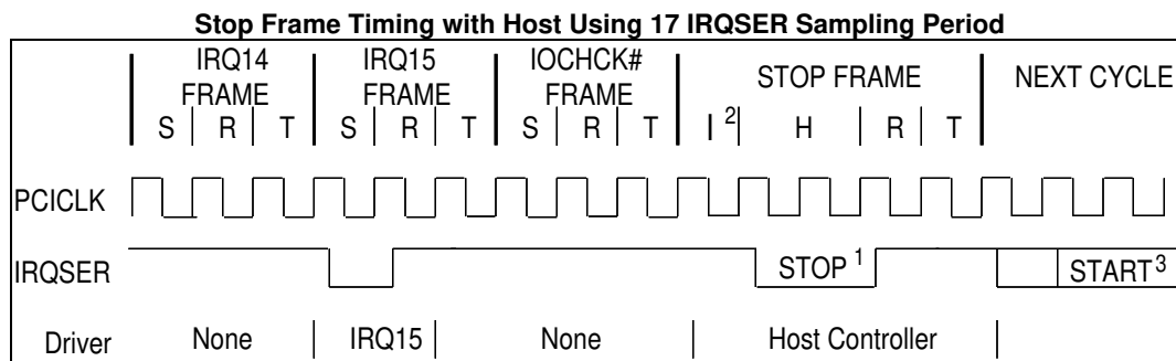
FIGURE 71 - SERIAL INTERRUPT WAVEFORM "STOP FRAME"
