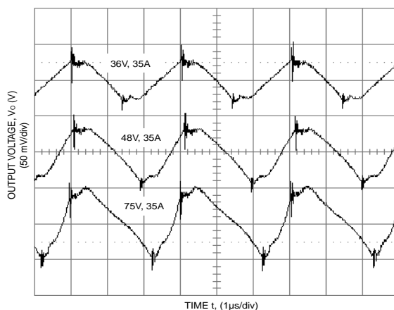
Figure 27. Output Ripple Voltage ( I_O = I_{O, \max} ).
