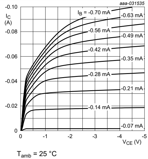
Fig. 5. NHDTA114EU: Collector current as a function of collector-emitter voltage; typical values
