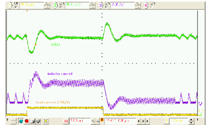
Figure 26. Load Transient, 3.6 V IN , 1.2 V OUT , 0.3–3 A, 100 ns Edge
