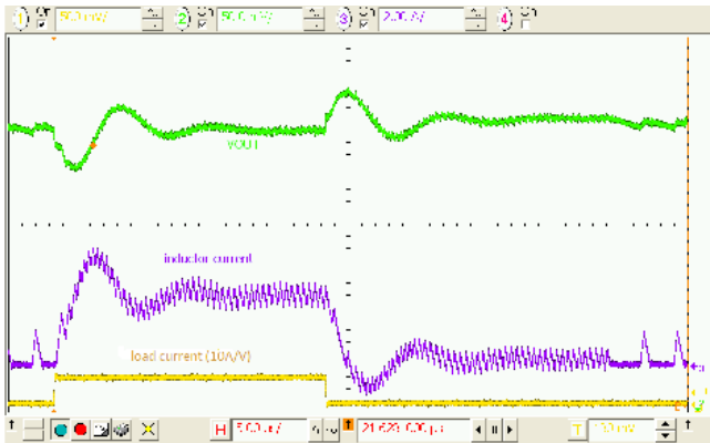
Figure 27. Load Transient, 3.6 V IN , 1.2 V OUT , 0.3–3 A, 100 ns Edge, C OUT = 4x22 μF
