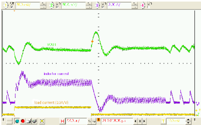
Figure 25. Load Transient, 5 V IN , 0.9 V OUT , 0.3–3 A, 100 ns Edge
