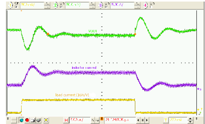
Figure 28. Load Transient, 3.6 V IN , 1.2 V OUT , 1.5–6 A, 100 ns Edge, C OUT = 4x22 μF
