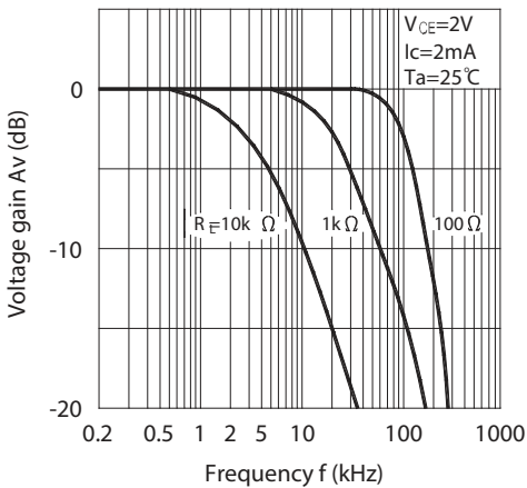
Figure 11: Frequency Response
