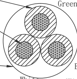
(Wire Cross-Section)
