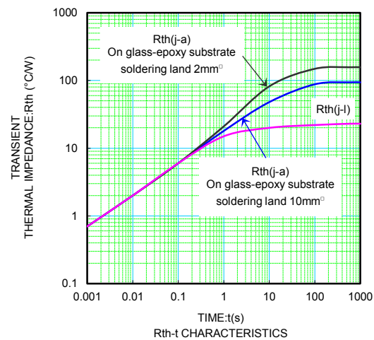
Rth-t CHARACTERISTICS
