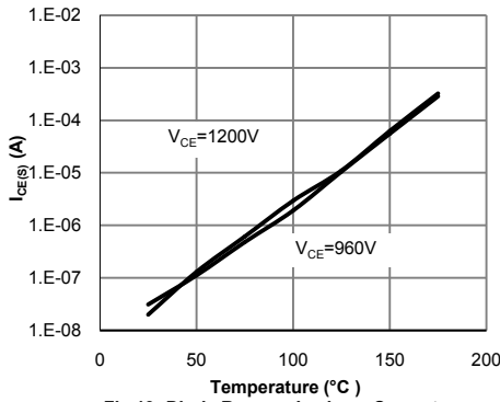
Fig 19: Diode Reverse Leakage Current vs. Junction Temperature
