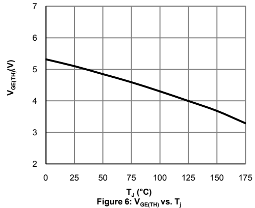
Figure 6: V_{GE(TH)} vs. T_j
