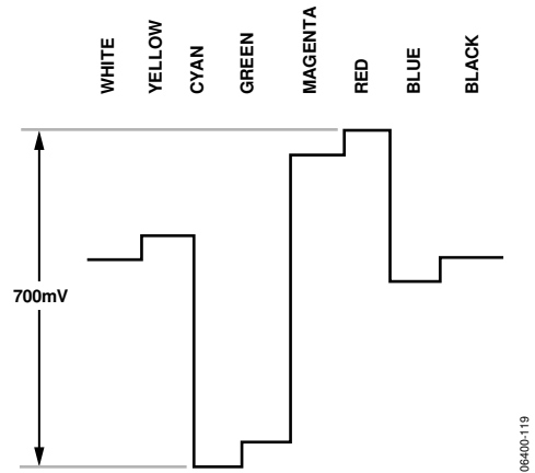
Figure 116. Pr Levels—PAL
