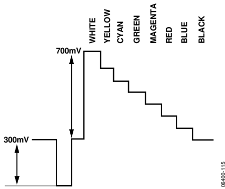
Figure 112. Y Levels—NTSC
