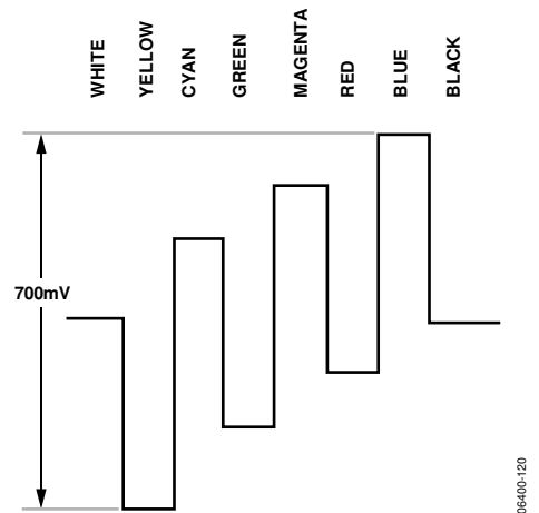
Figure 117. Pb Levels—PAL
