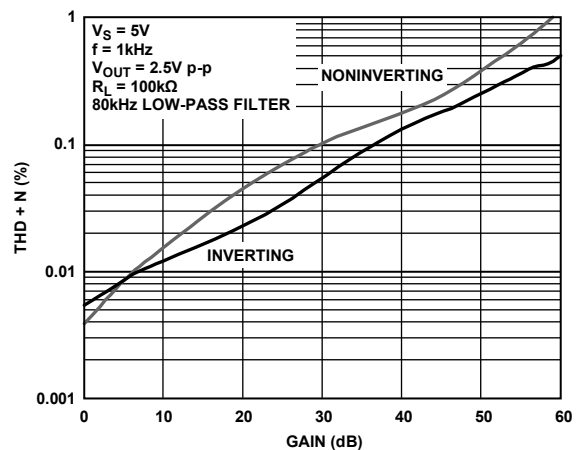
Figure 7. THD + N vs. Gain
