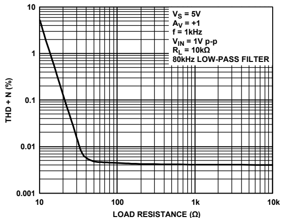
Figure 6. THD + N vs. Load (See Figure 3)
