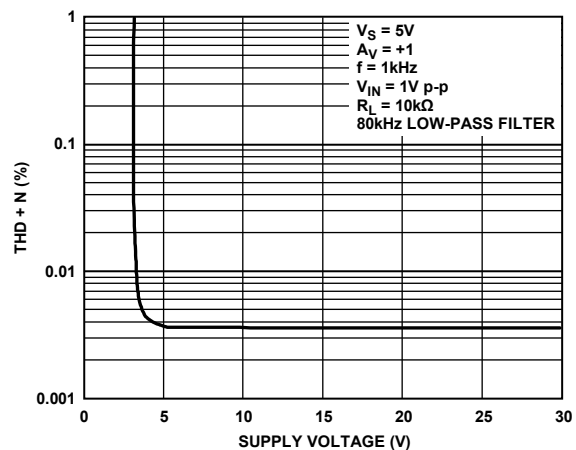
Figure 8. THD + N vs. Supply Voltage
