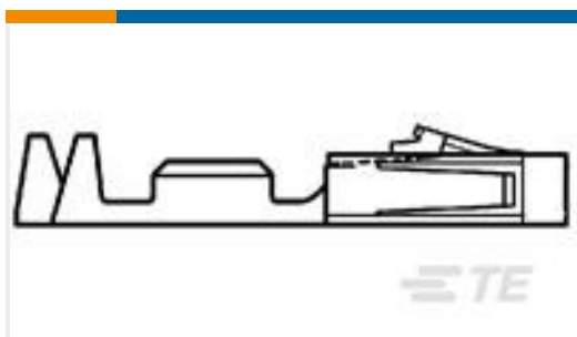
TE Part #104480-7 SHORT POINT RECP CONT LP
