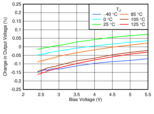
Figure 6-6. Output Accuracy vs V_{BIAS} and Temperature
