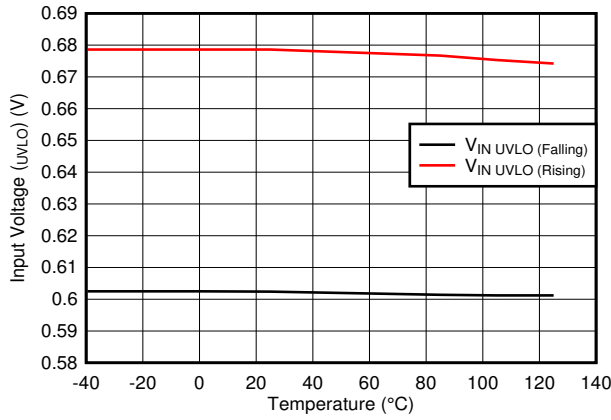
Figure 6-31. V UVLO(IN) Rising and Falling Threshold vs Temperature
