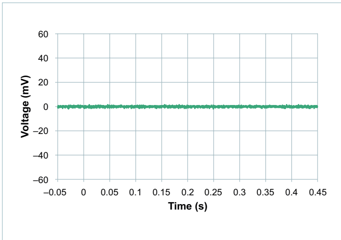
Figure 22 — AUX1 (-12V) ripple with 1A load, AC-coupled
