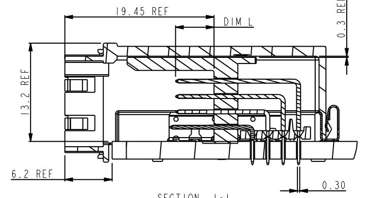
SECTION 1-1 SCALE 2.000
