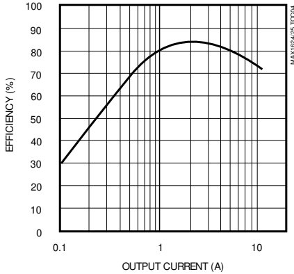
MAX1624 EFFICIENCY vs. OUTPUT CURRENT (V OUT = 1.1V)
