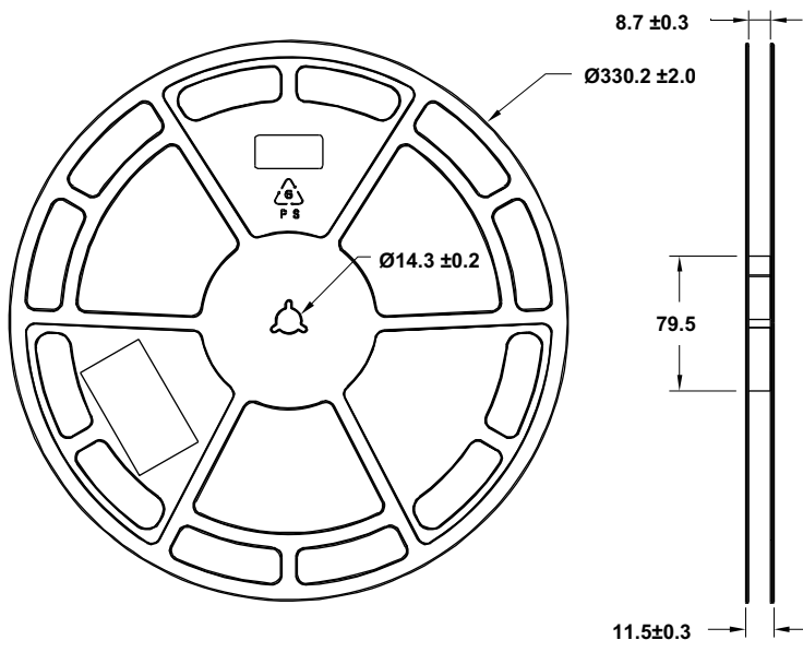
Figure 14: Reel Drawing
