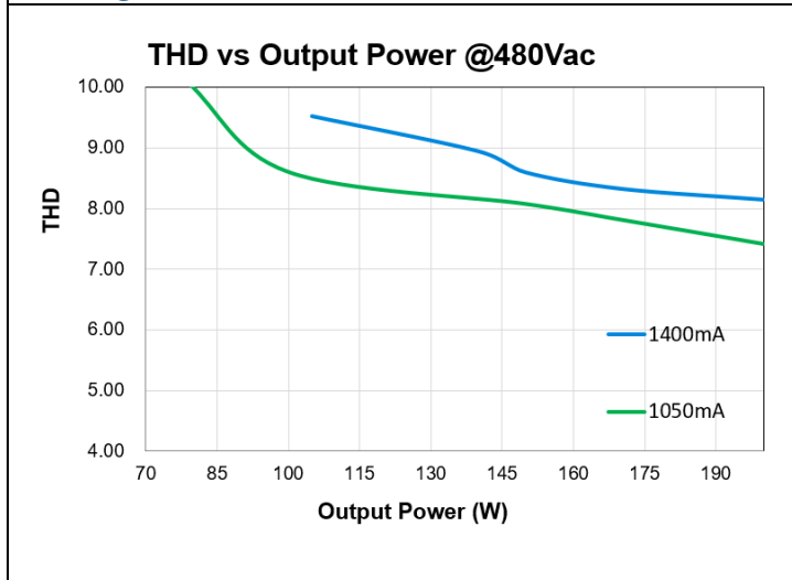
200W @ 480Vac
