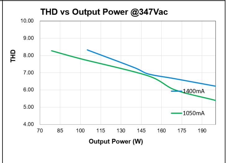
200W @ 347Vac
