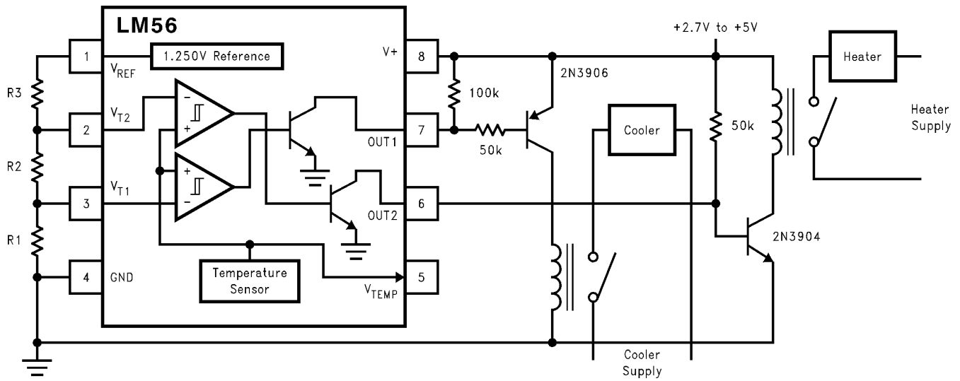
Figure 19. Simple Thermostat
