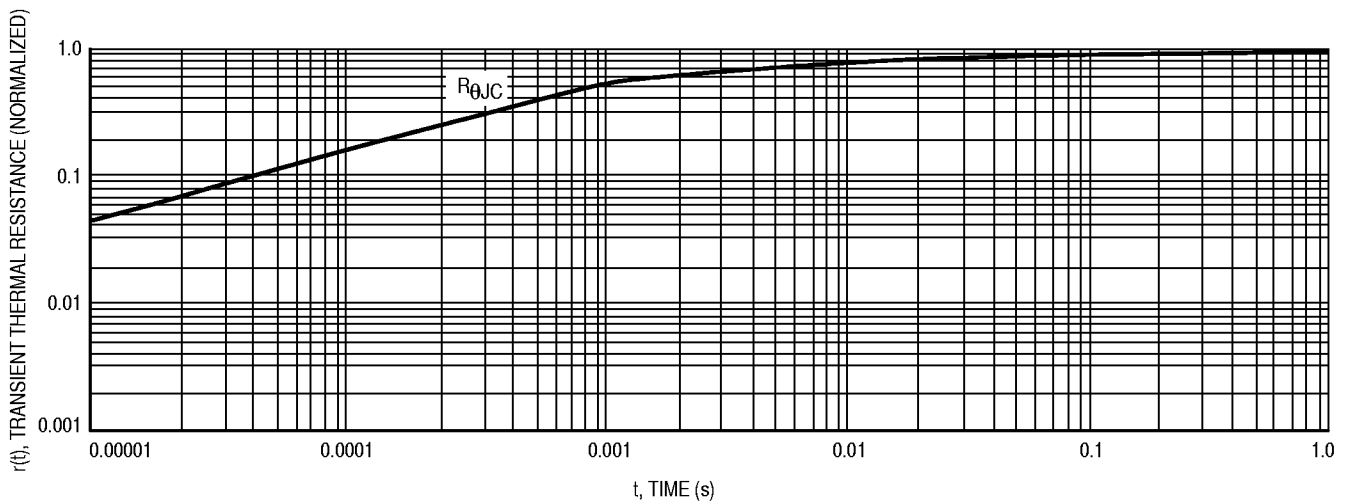
Figure 8. Thermal Response
