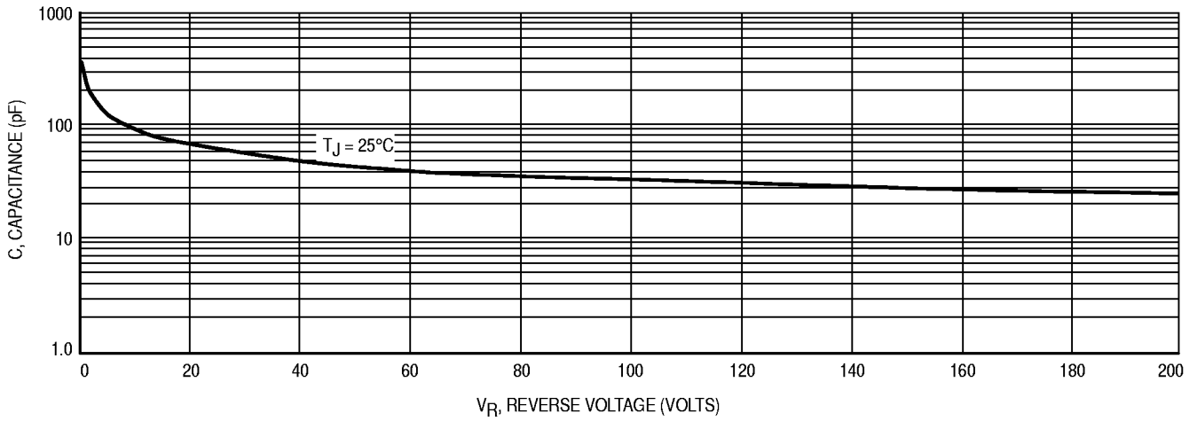
Figure 7. Capacitance
