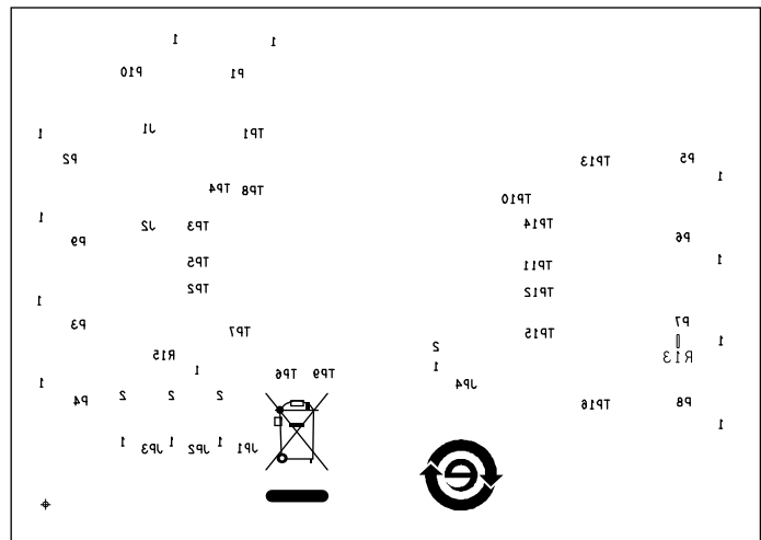
Figure 9. EVAL-ADM3055EEBZ Bottom Silkscreen
