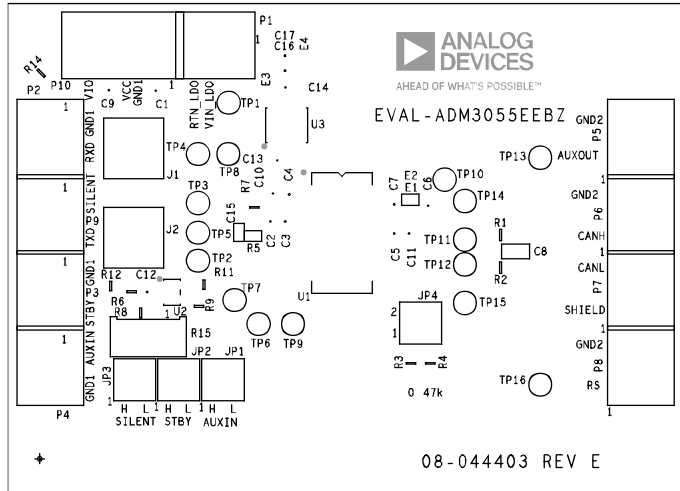
Figure 6. EVAL-ADM3055EBZ Primary Silkscreen
