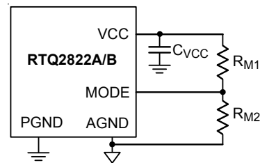
Figure 3. MODE Connection
