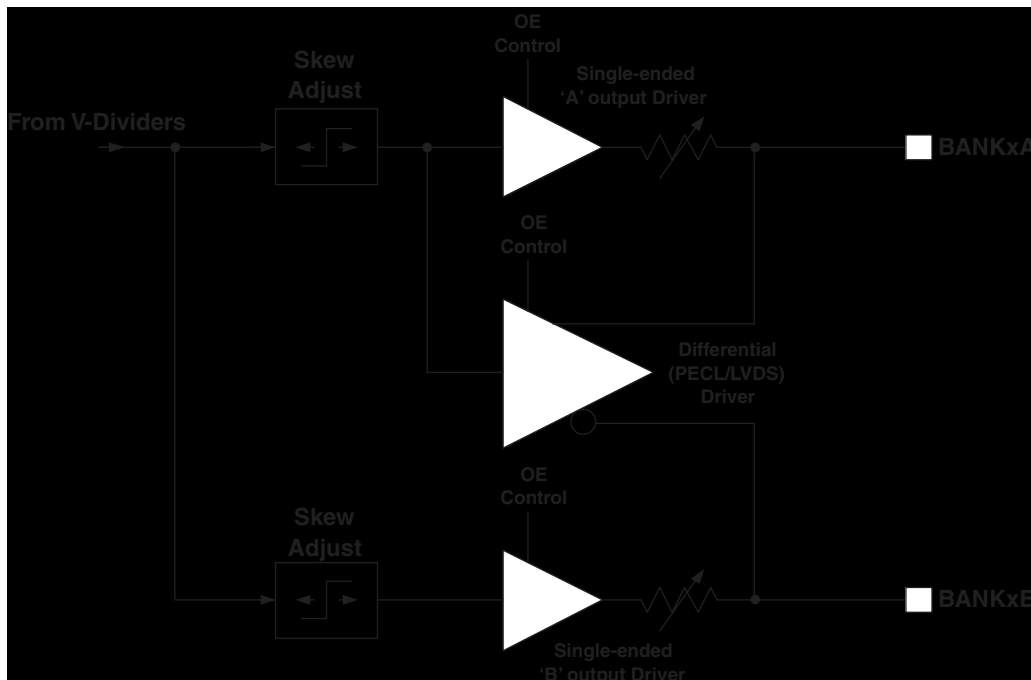
Figure 22. ispClock5500 Output Driver and Skew Control
