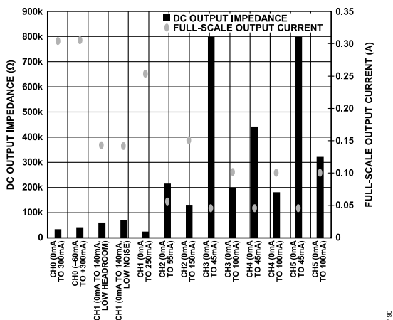
Figure 49. DC Output Impedance vs. Full-Scale Output Current (All Ranges)
