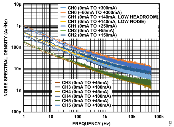
Figure 51. Output NSD vs. Frequency (All Ranges)
