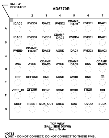
Figure 4. Pin Configuration
