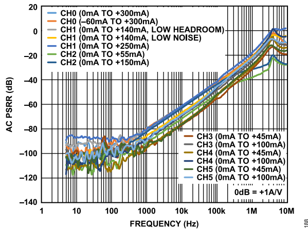
Figure 48. AC PSRR vs. Frequency (All Ranges)
