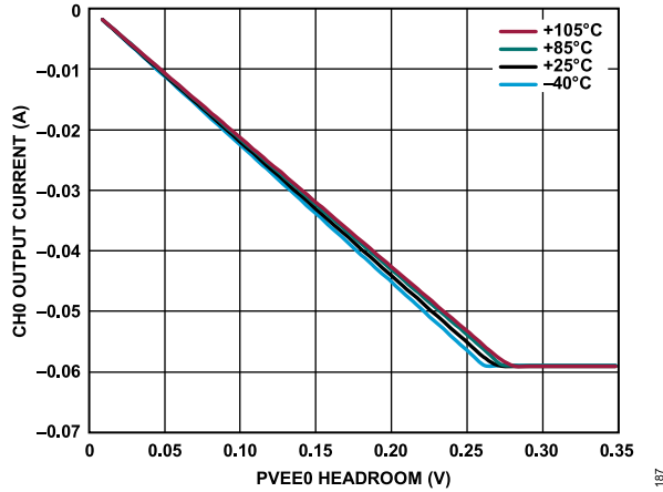
Figure 47. CH0 Output Current vs. PVEE0 Footroom for Various Temperatures
