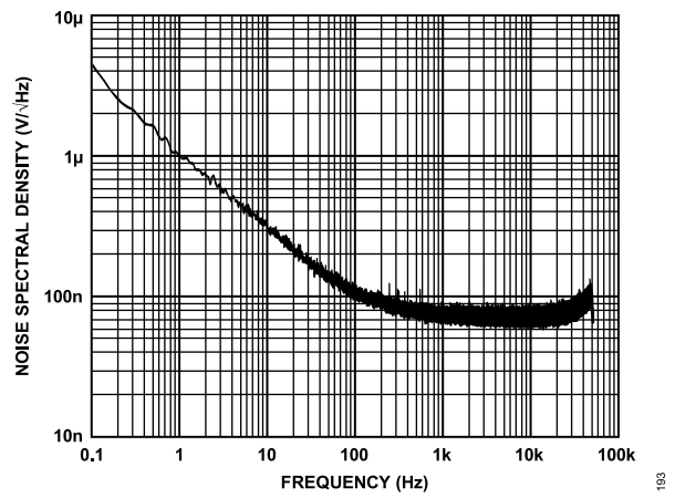
Figure 52. VREF_IO Output NSD vs. Frequency
