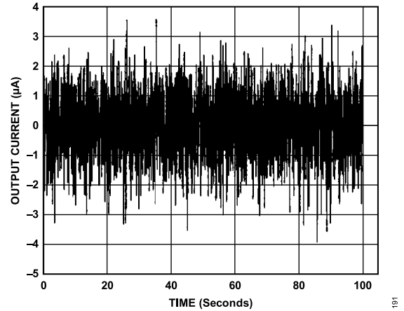
Figure 50. Peak-to-Peak Noise, 0.1 Hz to 10 Hz Bandwidth, (CH0 0 mA to 300 mA Range)
