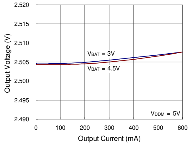
CH3 Step-Down Output Voltage vs. Output Current
