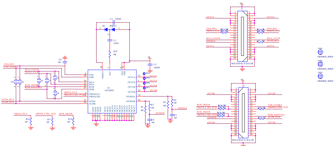
Figure 7. EVL6226-PLUG
