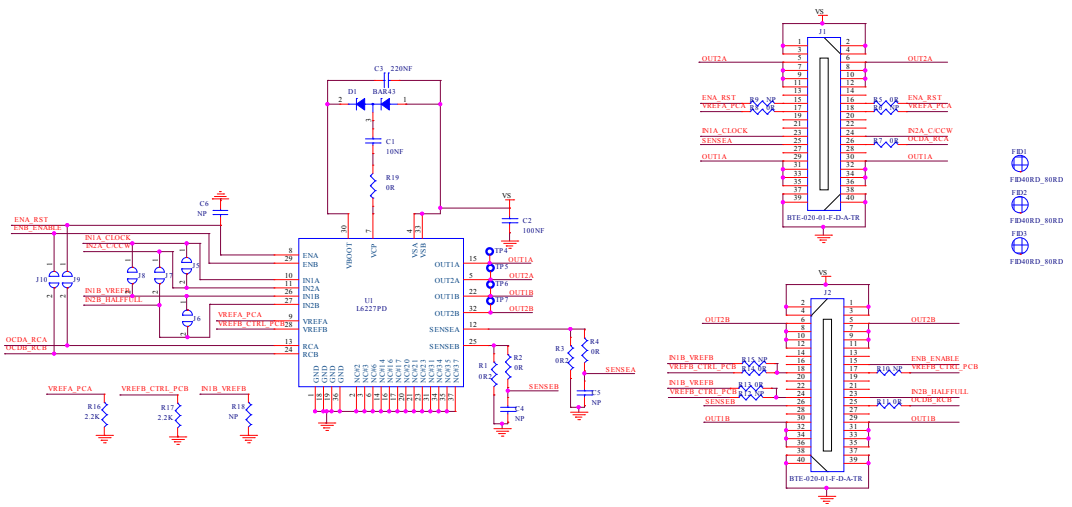
Figure 8. EVL6227-PLUG
