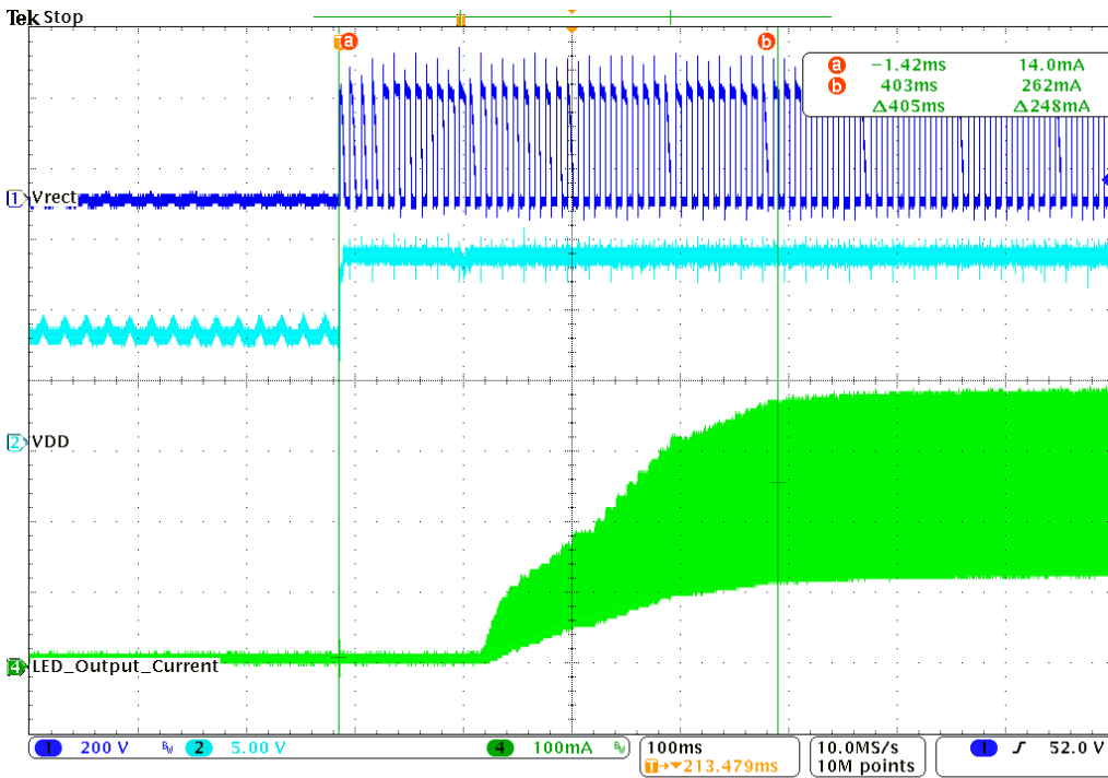
Figure 22. ILED at Medium Dim Angle, Turn-on Waveforms
