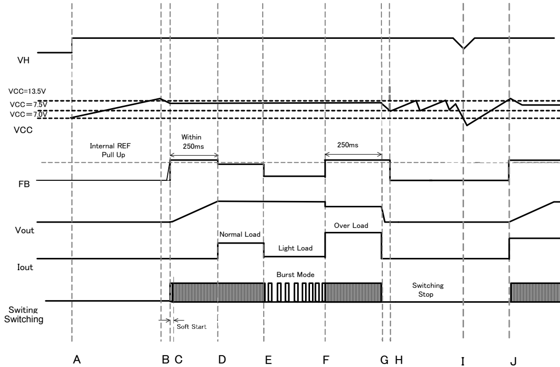
Figure 5, Start Sequence Timing Chart
