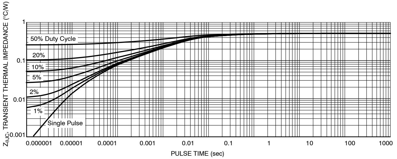
Figure 13. Thermal Characteristics
