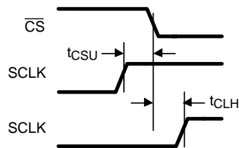
Figure 4. SCLK and CS Timing Parameters
