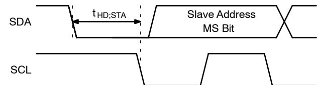
Figure 24. Start Bit
