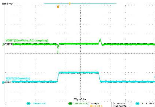
Figure 20. LDO3/4 Load Transient, V_{\text{IN}} = 3.8\text{ V} , V_{\text{OUT}} = 2.8\text{ V} , 1\text{ mA} \leftrightarrow 200\text{ mA} , 2\text{ }\mu\text{s} Edge
