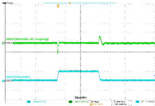
Figure 22. LDO6/7 Load Transient, V_{\text{IN}} = 3.8\text{ V} , V_{\text{OUT}} = 2.8\text{ V} , 1\text{ mA} \leftrightarrow 200\text{ mA} , 2\text{ }\mu\text{s} Edge
