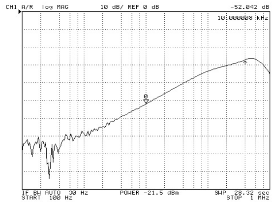
Figure 11. LDO1/2 PSRR vs. Frequency, 150 mA Load
