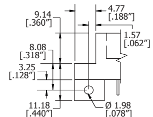
STRADDLE MOUNT (Q)
