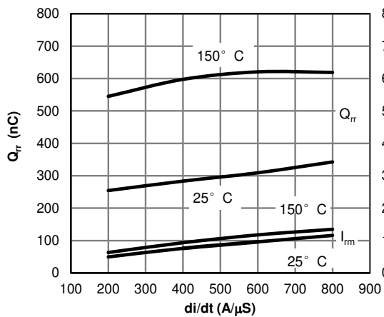
Figure 24: Diode Reverse Recovery Charge and Peak Current vs. di/dt ( V_{GE}=15V, V_{CE}=400V, I_F=10A )
