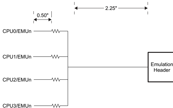
Figure 26. Parallel Termination
