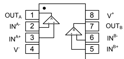
SO-8 / MSOP-8
