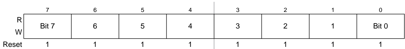
Figure 12-25. PWM Channel Duty Registers (PWMDTY2)
