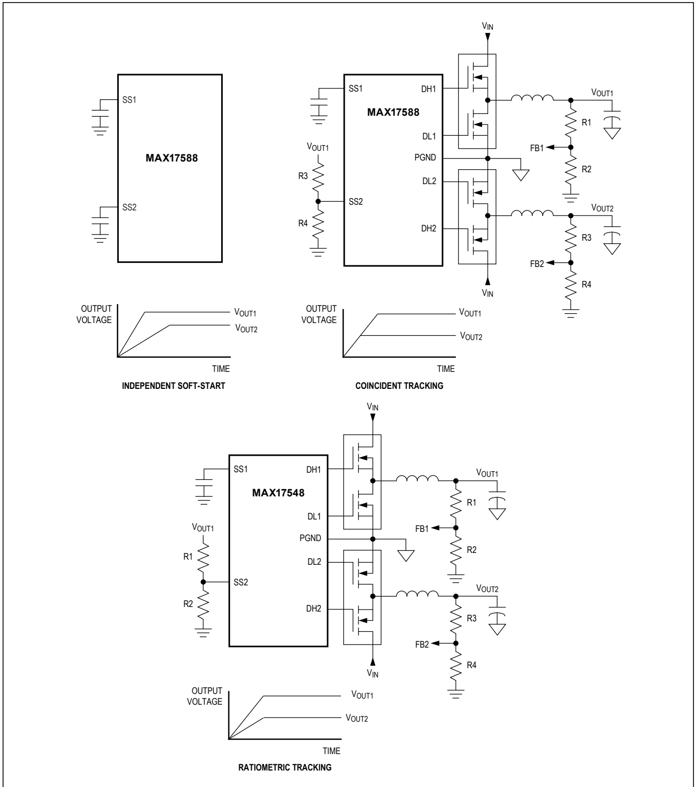
Figure 2. Possible SS i Pin Configurations
