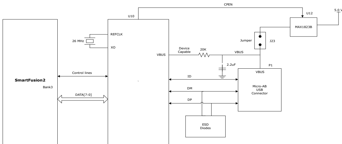
Figure 11 • USB Interface
