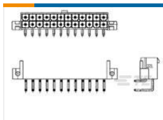
TE Part #1586044-4 4P VAL-U-LOK R/A HDR SCR MT V0
