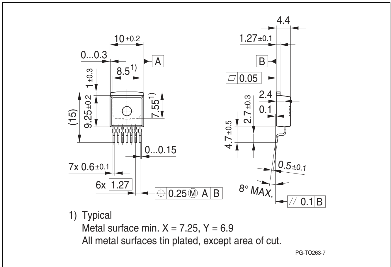
Figure 14 PG-T0263-7
