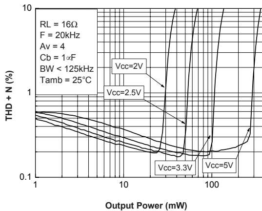
Figure 63. THD + N vs. output power RL = 16 Ω
