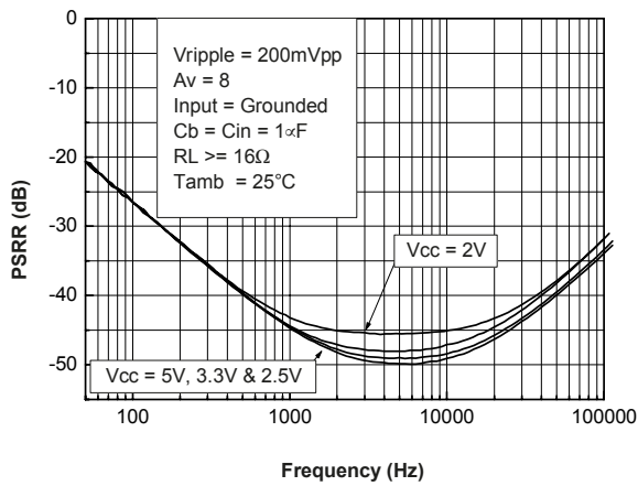
Figure 95. PSRR vs. bypass capacitor C_b = C_{in} = 1 \mu F
