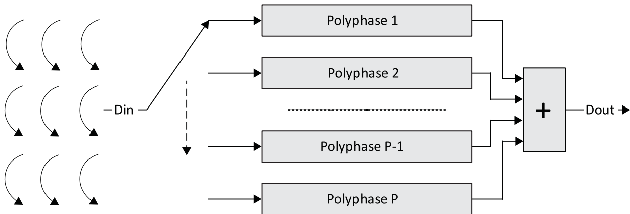
Figure 4.5. Polyphase Decimator
