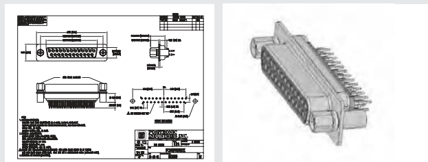
2-D Drawing
