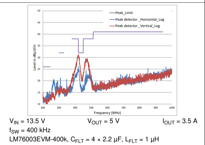
Figure 88. LM76003-Q1 Radiated EMI Result vs. CISPR25 Limits - High Frequency
