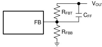
Figure 19. Feed-Forward Capacitor for Loop Compensation
