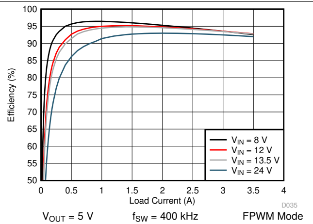
Figure 26. LM76003-Q1 Efficiency
