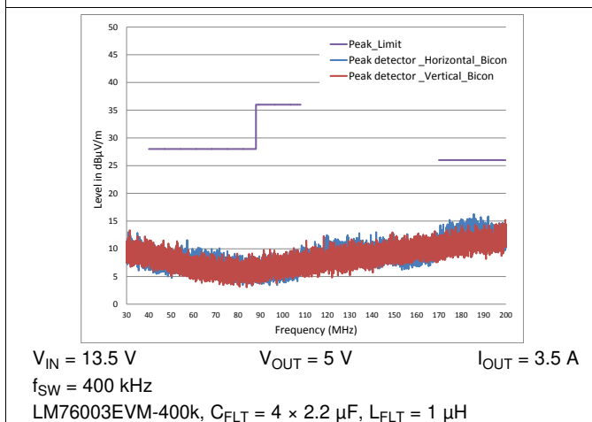
Figure 87. LM76003-Q1 Radiated EMI Result vs. CISPR25 Limits - Low Frequency
