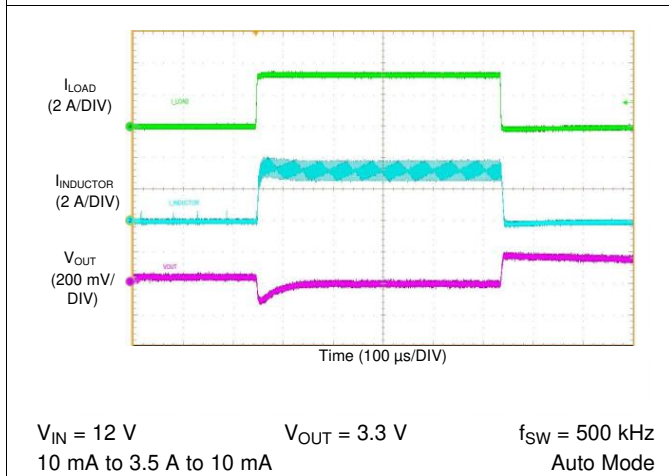
Figure 73. LM76003-Q1 Load Transient
