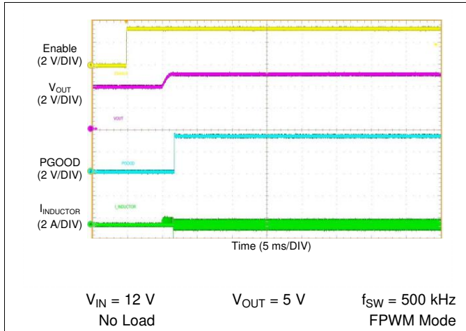
Figure 71. LM76002-Q1 Start-up With Pre-Biased Output
