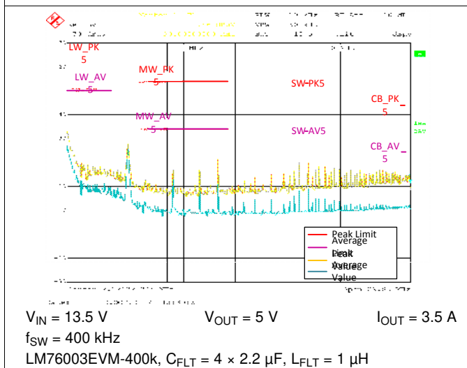
Figure 85. LM76003-Q1 Conducted EMI Result vs. CISPR25 Limits - Low Frequency
