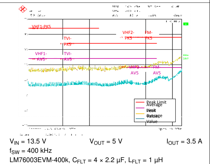
Figure 86. LM76003-Q1 Conducted EMI Result vs. CISPR25 Limits - High Frequency
