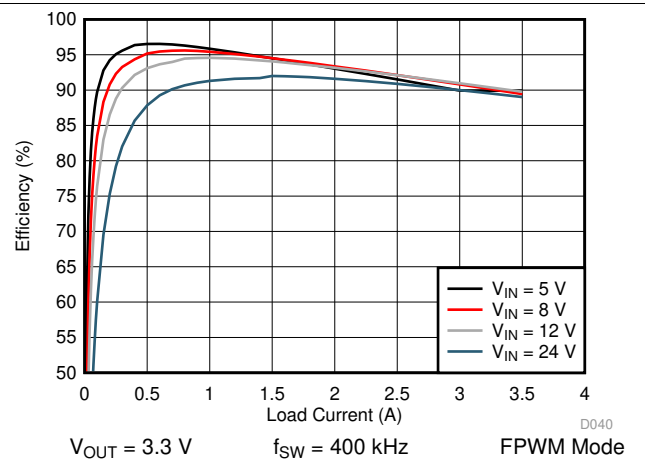
Figure 24. LM76003-Q1 Efficiency
