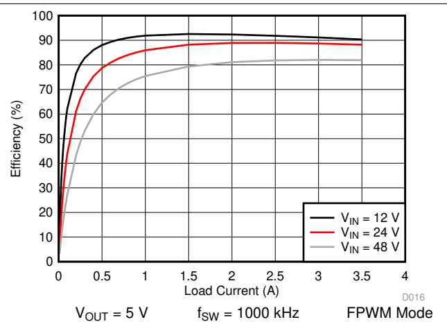
Figure 28. LM76003-Q1 Efficiency
