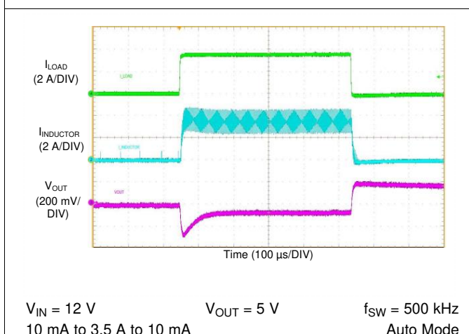
Figure 75. LM76003-Q1 Load Transient
