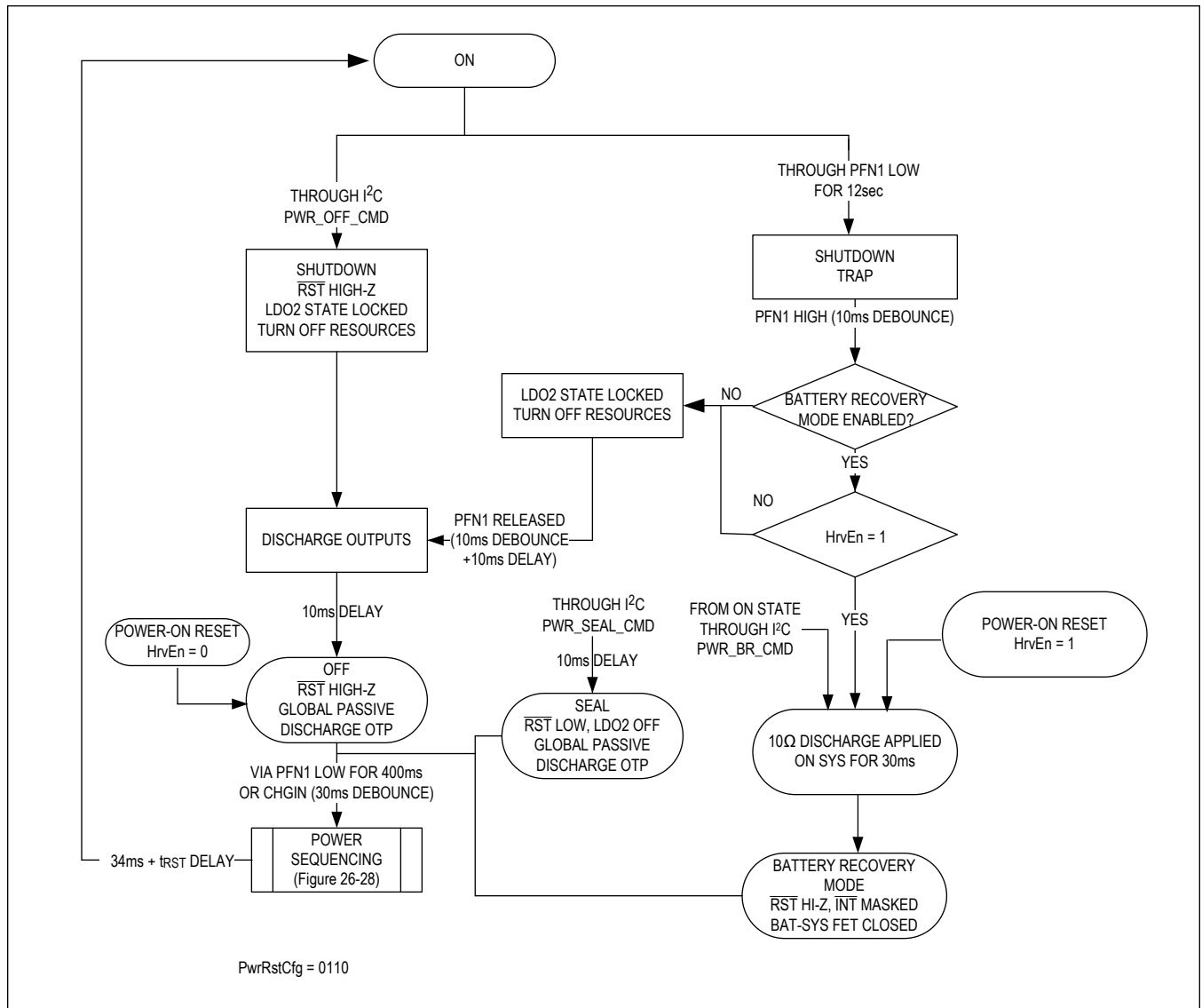
Figure 18. PwrRstCfg 0110
