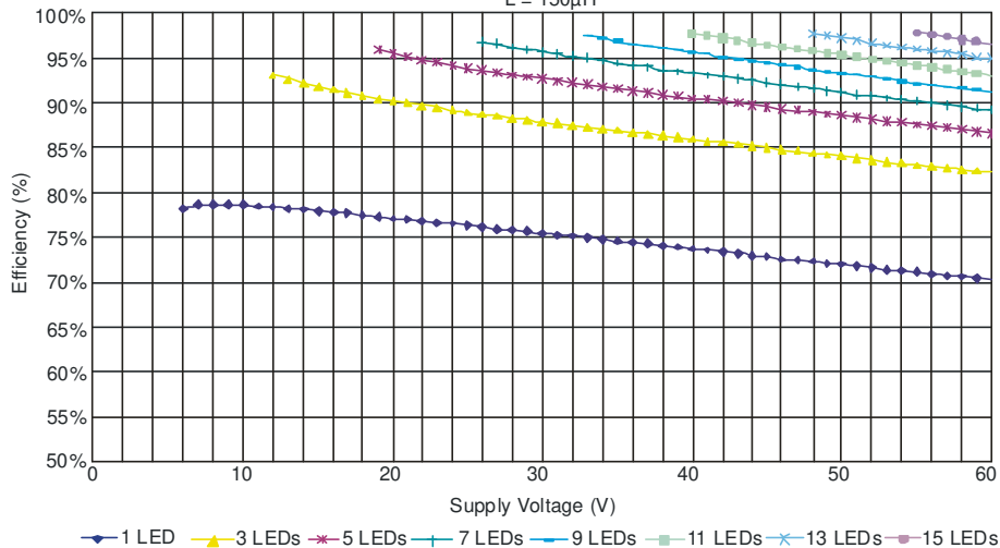
ZXLD1356Q Efficiency L = 150μH
