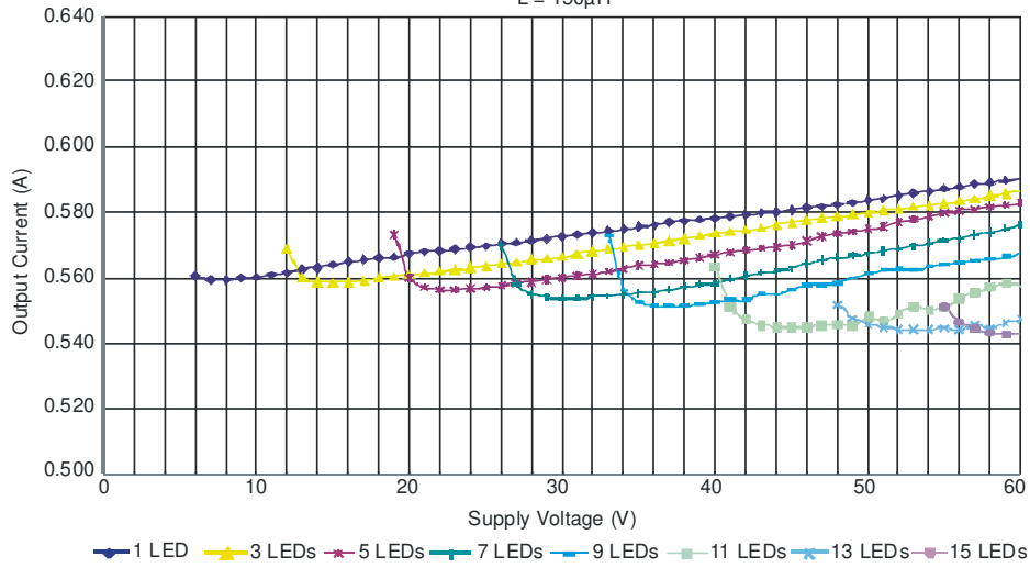
ZXLD1356Q Output Current Deviation (Normalized) L = 150μH
