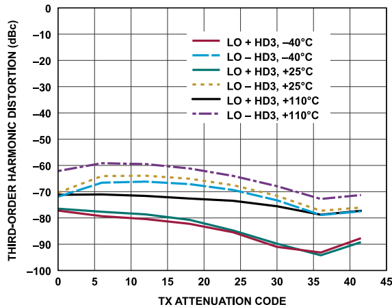
Figure 257. Transmitter Third-Order Harmonic Distortion vs. Transmitter Attenuation Code, Baseband Frequency = 2.1 kHz, Backoff = 0.2 dBFS
