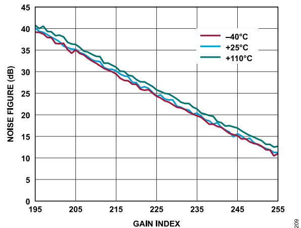
Figure 110. Receiver Noise Figure vs. Gain Index, Baseband Frequency = 5.6 MHz, ADC = High Performance
