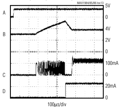
STARTUP WAVEFORMS
