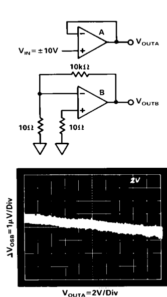
Figure 24. Crosstalk with No Load
