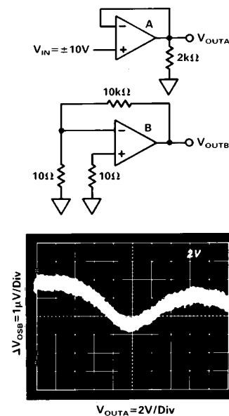
Figure 25. Crosstalk with 2 kΩ Load
