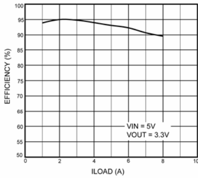
MIC2168A Efficiency
